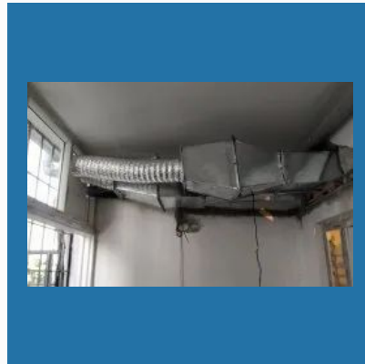
Toilet Exhaust Ducting
